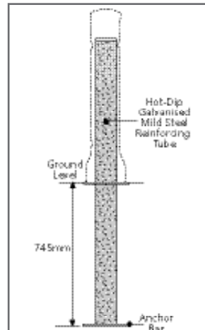
Below-Ground Guardsman™ Anti-Ram Raid
